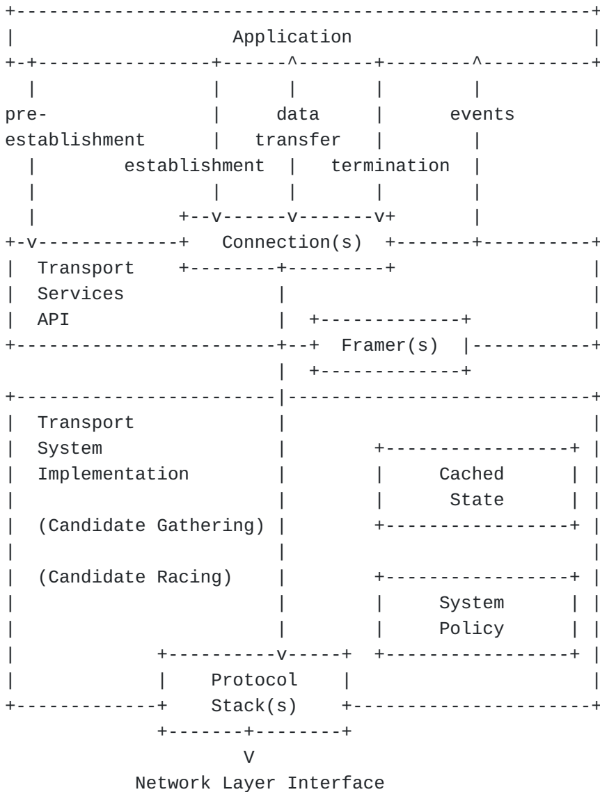
Figure 3: Concepts and Relationships in the Transport Services Architecture
