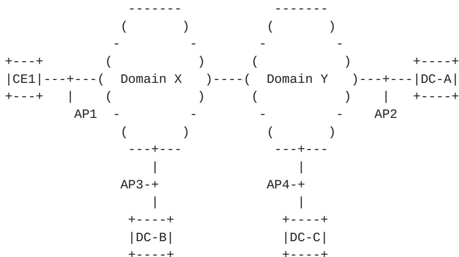
Figure 14: End-Point Selection Based on Network Status
