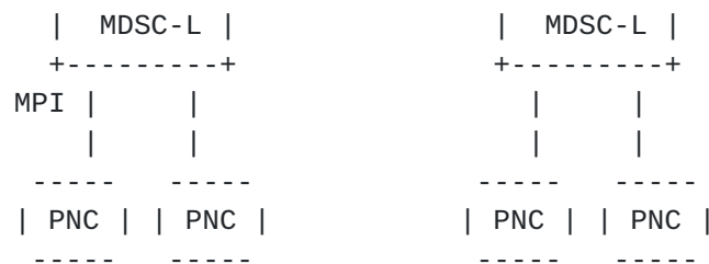
Figure 4: MDSC Hierarchy
