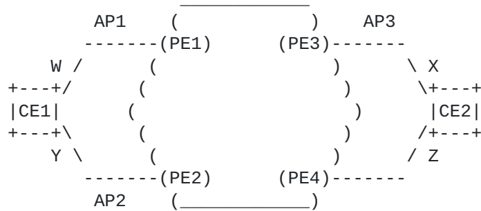
Figure 12: Dual-Homing Scenario
