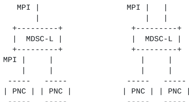
Figure 4: MDSC Hierarchy
