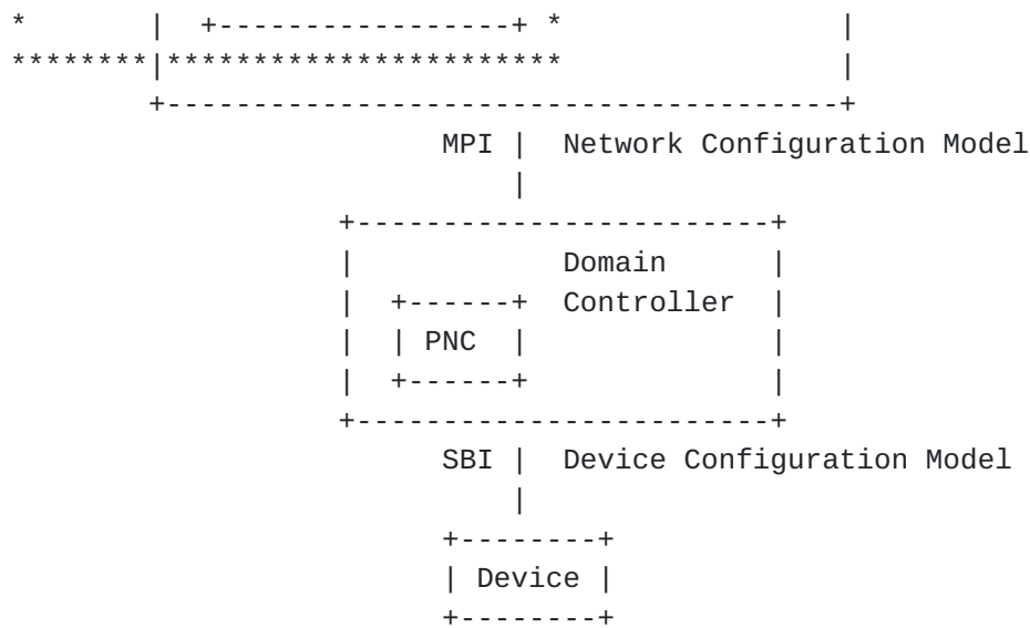
Figure 5: ACTN Architecture in the Context of the YANG Service Models
