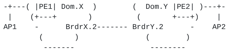
Figure 8: A Multi-Domain Example
