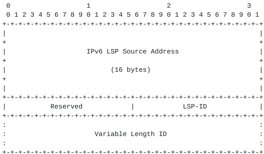
Figure 5: IPv6 Extended Association ID Format Example
