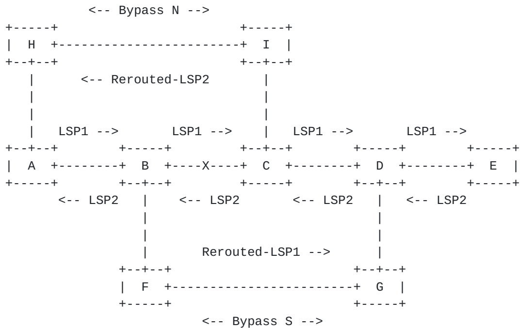
Figure 2: Node Protection Bypass Tunnels
