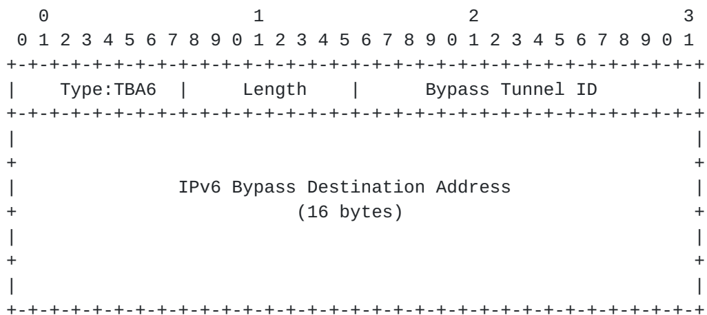
Figure 5: BYPASS_ASSIGNMENT IPv6 RR0 Subobject
