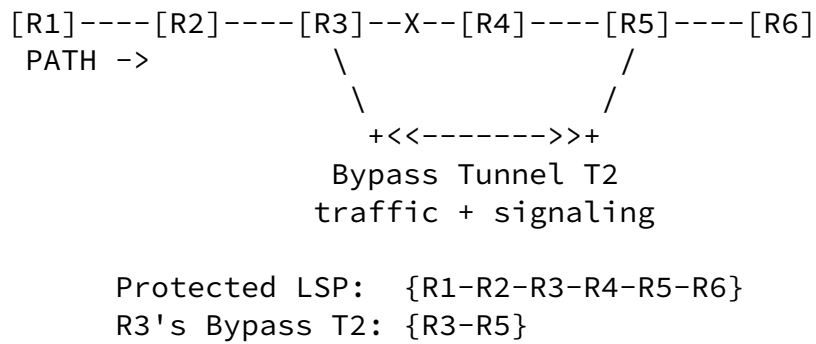
Figure 3: Flow of RSVP signaling after FRR and re-coroute
