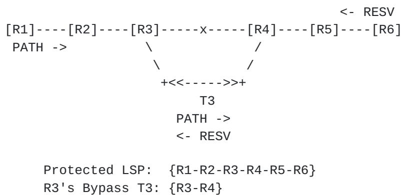
Figure 1: Flow of RSVP signaling after link failure and FRR
