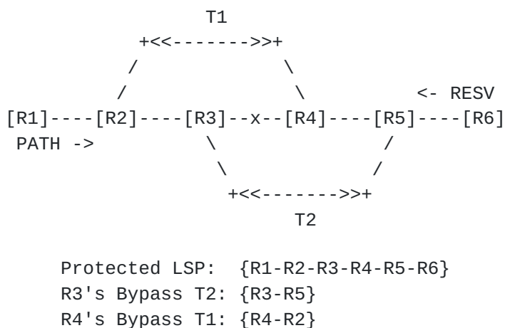
Figure 2: Flow of RSVP signaling after link failure and FRR
