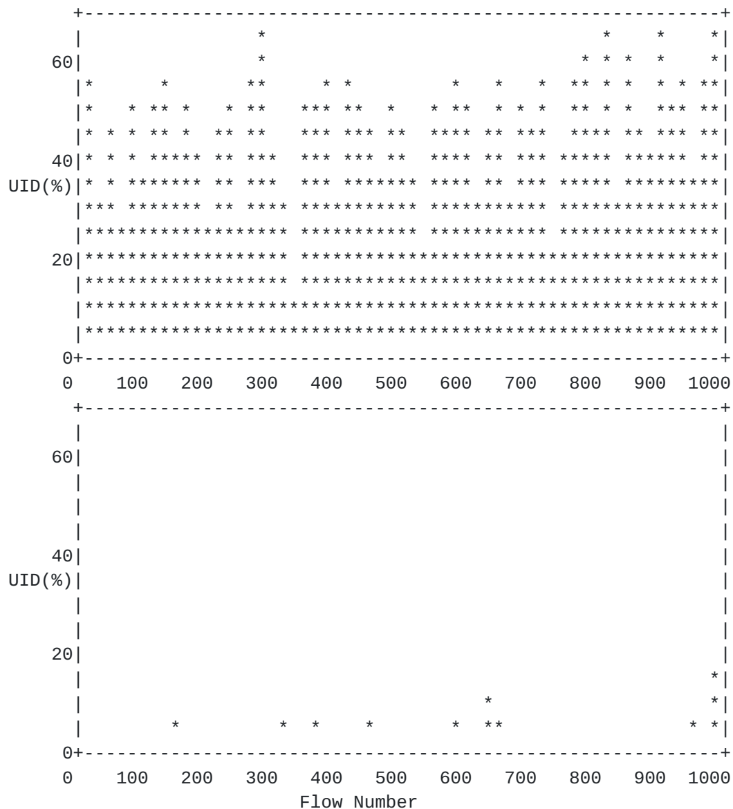
Figure 6: Simulation Result with Congestion Elimination
