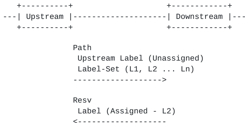
Figure 2: Signaling Sequence
