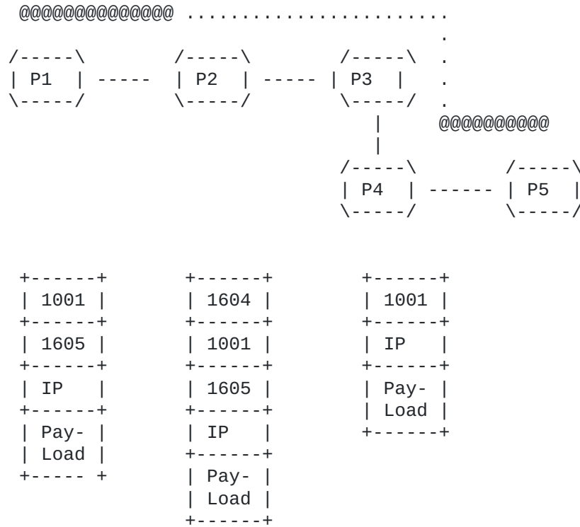
Figure 5: Extending network slice over NRP incapable device(s).
