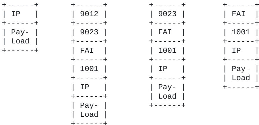
Figure 4: FAI and FAS label in the label stack.
