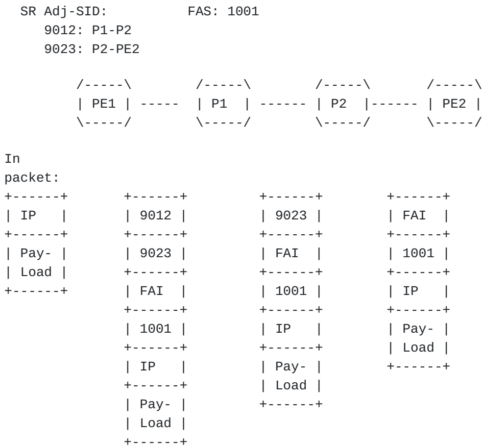
Figure 4: FAI and FAS label in the label stack.
