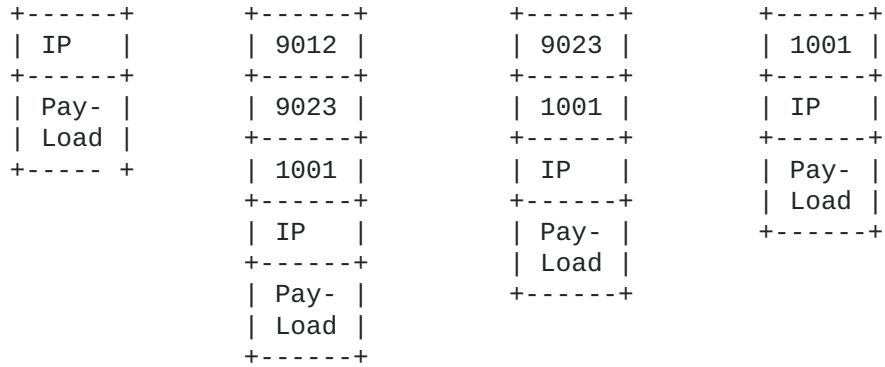
Figure 3: FAS or VPN label at bottom of label stack.
