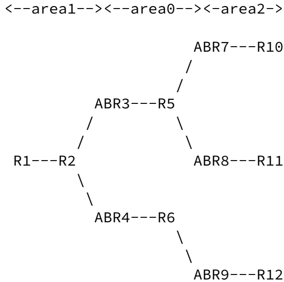
Figure 1: An Example of Loosely Routed Inter-domain P2MP-TE LSP Tree
