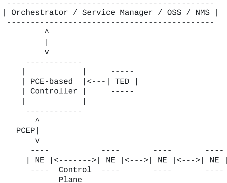
Figure 1: Architecture for Central Controller with Control Plane
