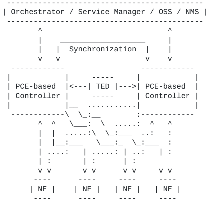
Figure 5: Multiple Redundant Controllers
