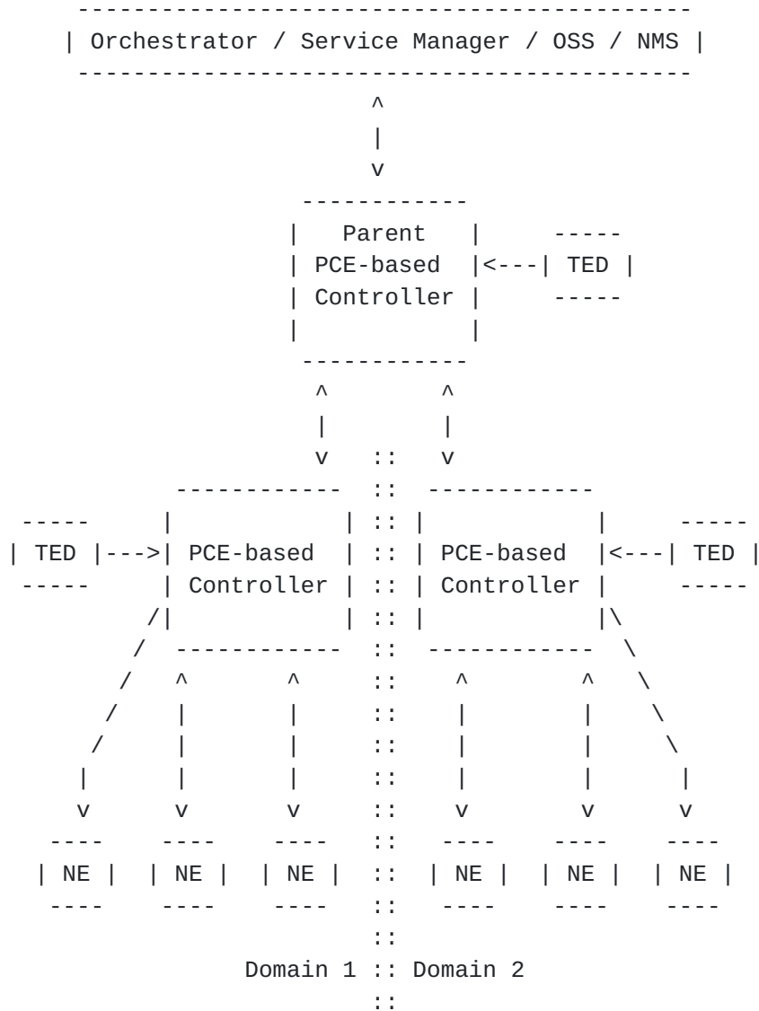
Figure 6: Hierarchical Controllers
