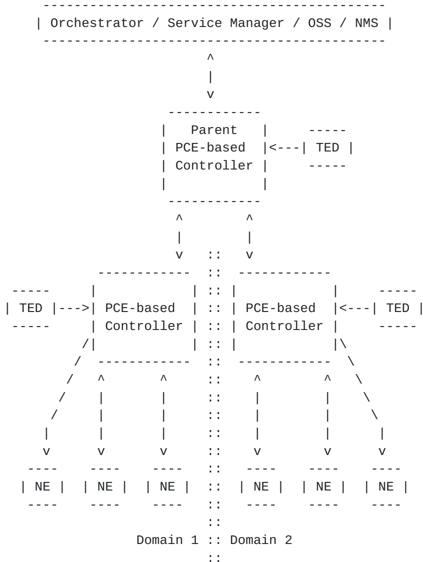
Figure 7: Hierarchical Controllers
