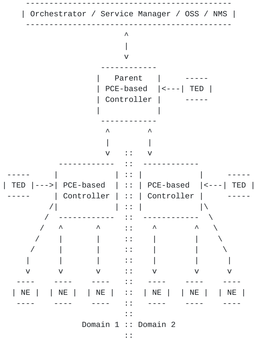
Figure 7: Hierarchical Controllers
