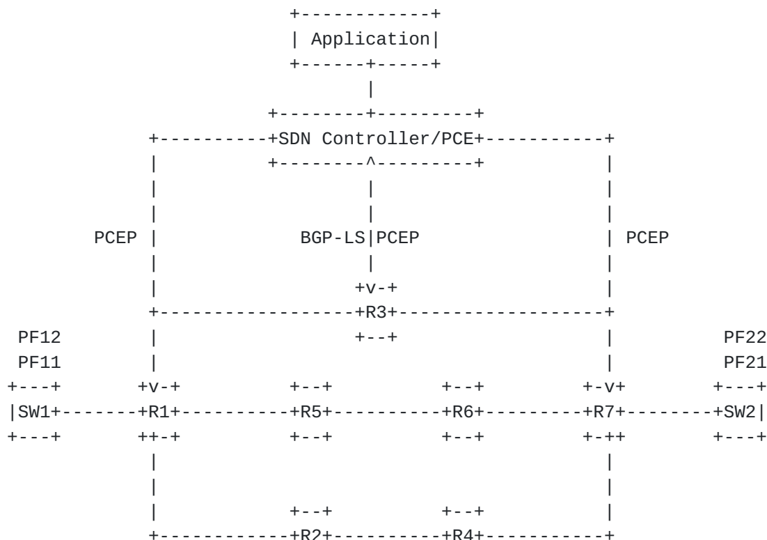
Figure 3: CCDD architecture for Multi-BGP deployment
