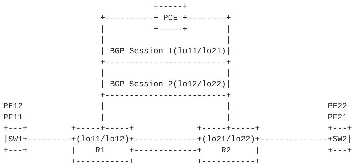
Figure 1: CCDD architecture in simple topology
