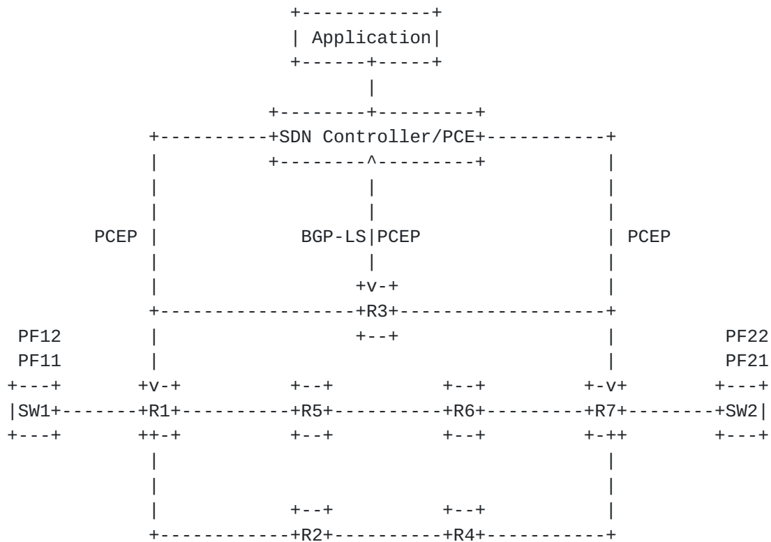
Figure 3: CCDR architecture for Multi-BGP sessions deployment
