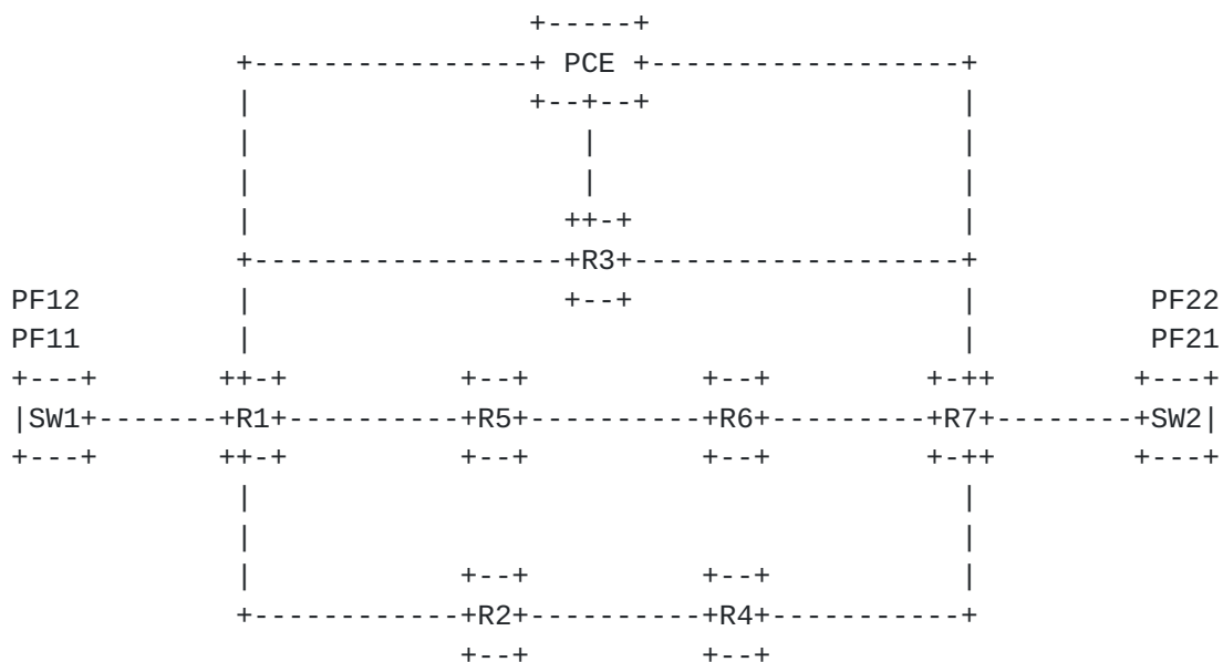
Figure 2: CCDD architecture in large scale network
