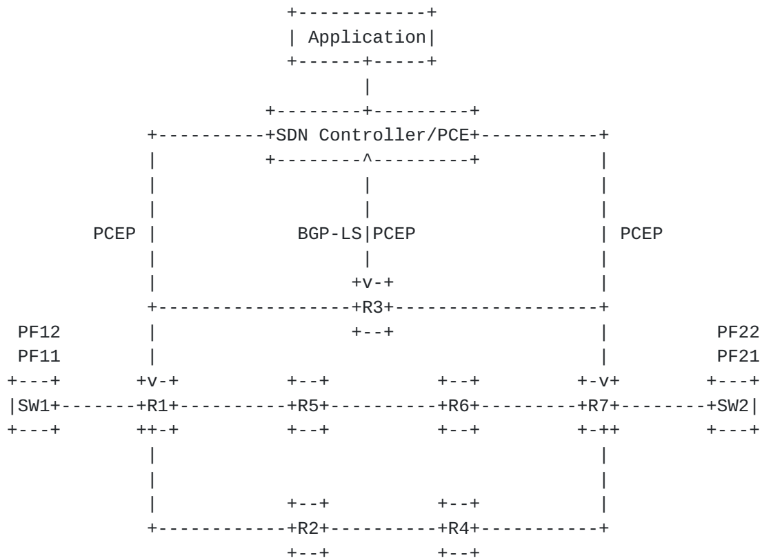
Figure 3: CCDD architecture for Multi-BGP sessions deployment
