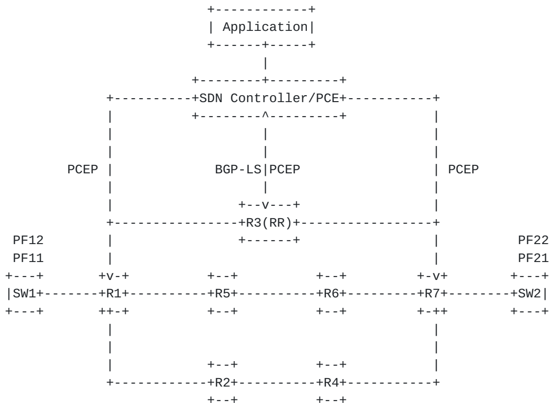
Figure 3: CCDR architecture for Multi-BGP sessions deployment
