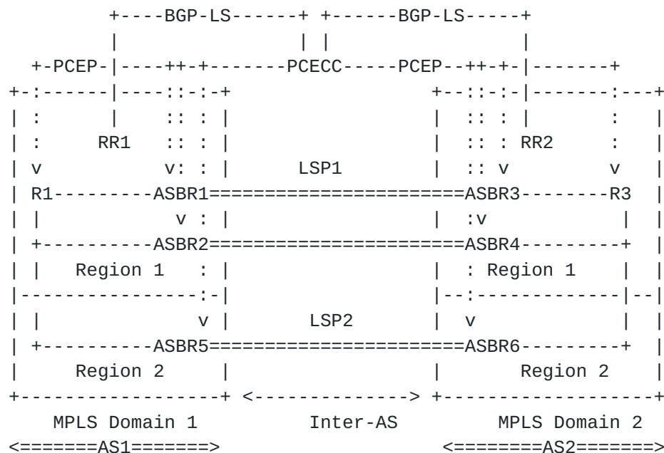
Particular case of Inter-AS PCE
