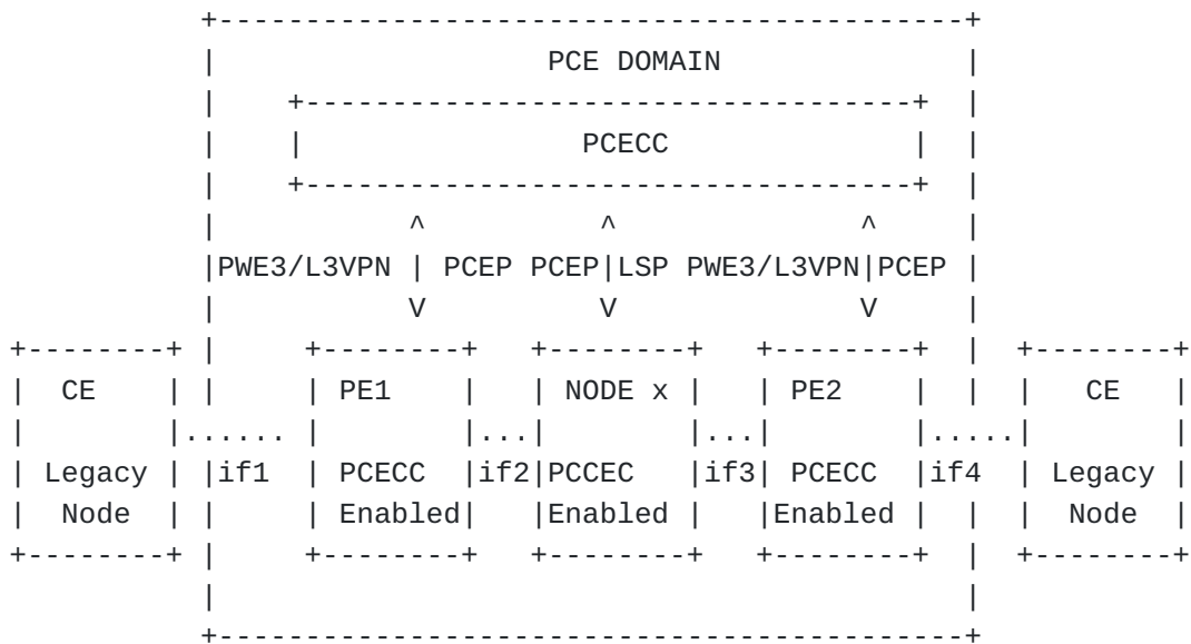
Example: Using PCECC for L3VPN and PWE3
