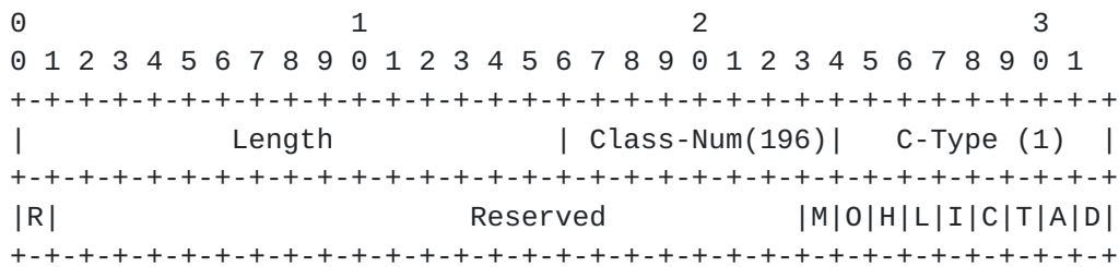
Figure 1. Admin_Status Object
