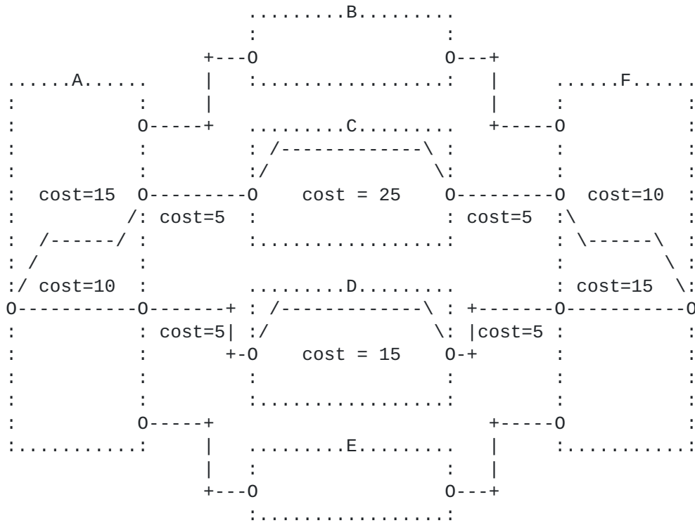
Figure 10 - Multi-domain with many domains (Path Computation information)
