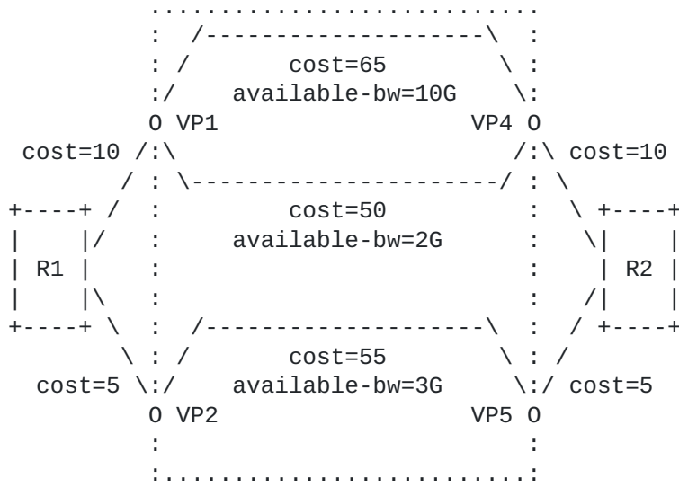
Figure 8 - Packet/Optical Path Computation Example with multiple choices
