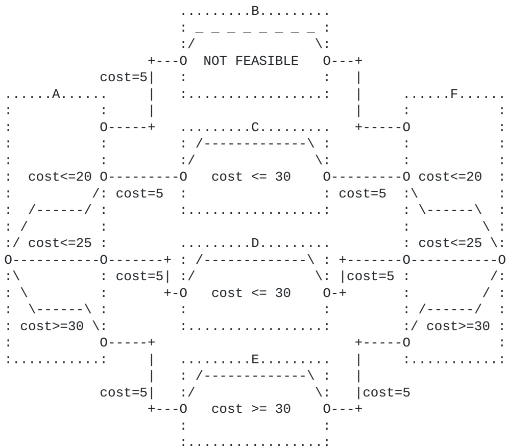
Figure 9 - Multi-domain with many domains (Topology information)
