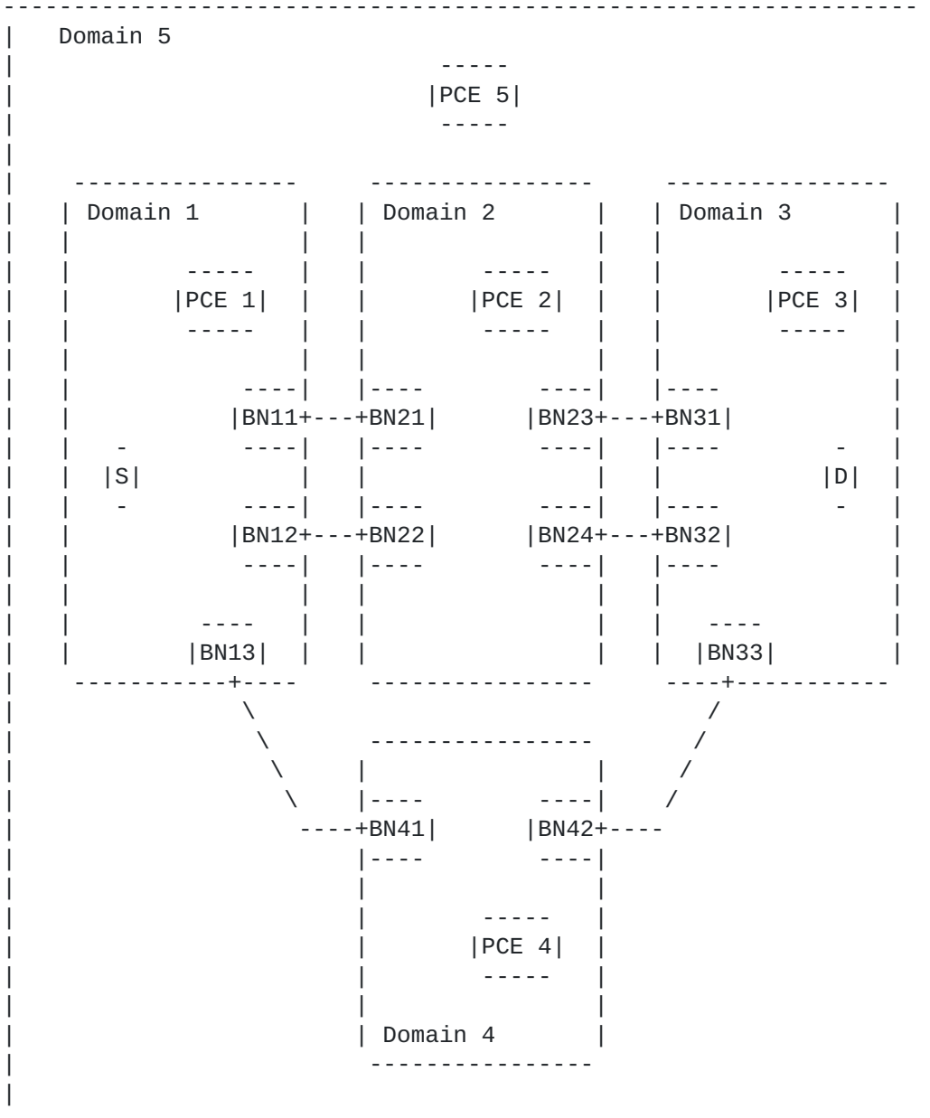
Figure 7 - Hierarchical domain topology from [ RFC6805 ]
