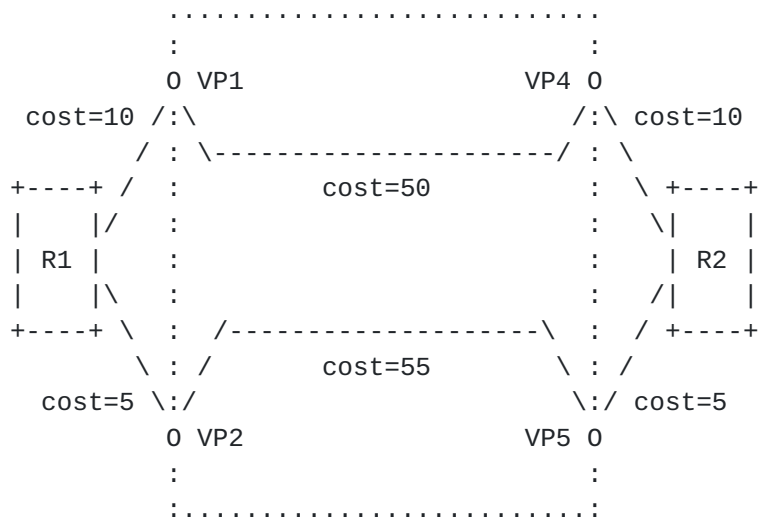
Figure 3 - Packet/Optical Path Computation Example
