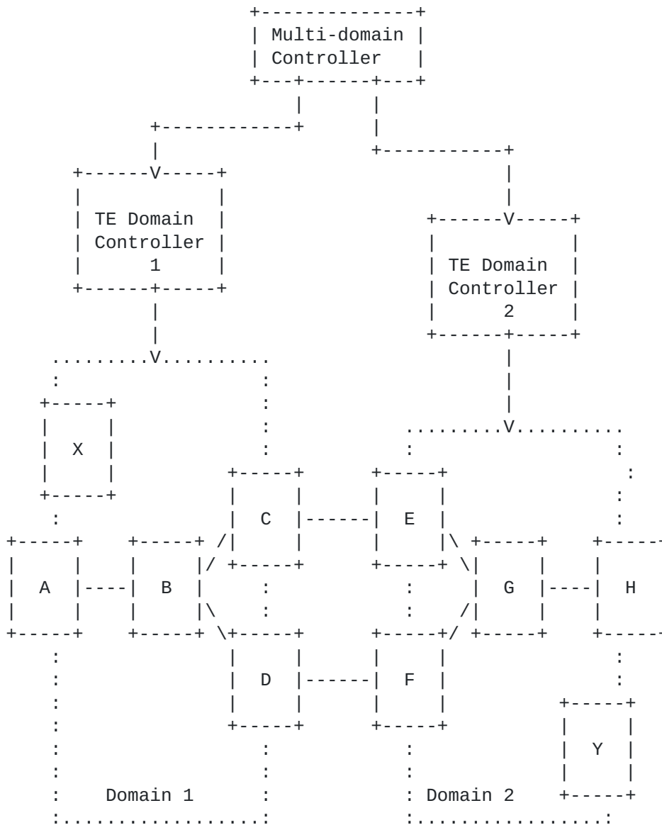
Figure 4 - Multi-domain multi-link interconnection
