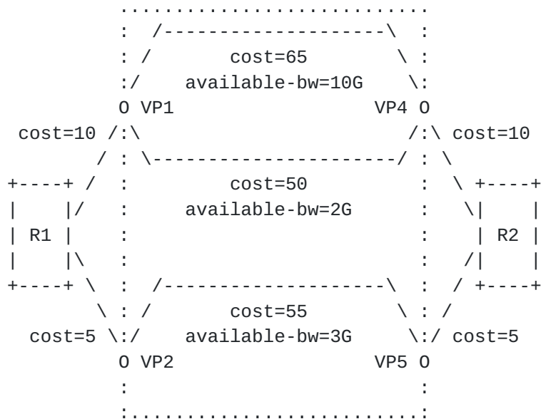
Figure 8 - Packet/Optical Path Computation Example with multiple choices
