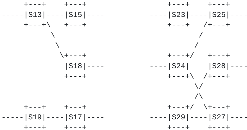
Figure 9: Merging Domain TE Topologies
