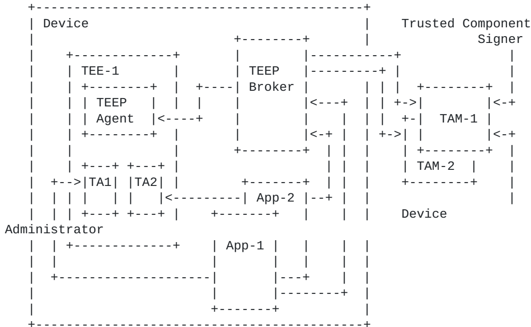
Figure 1: Notional Architecture of TEEP
