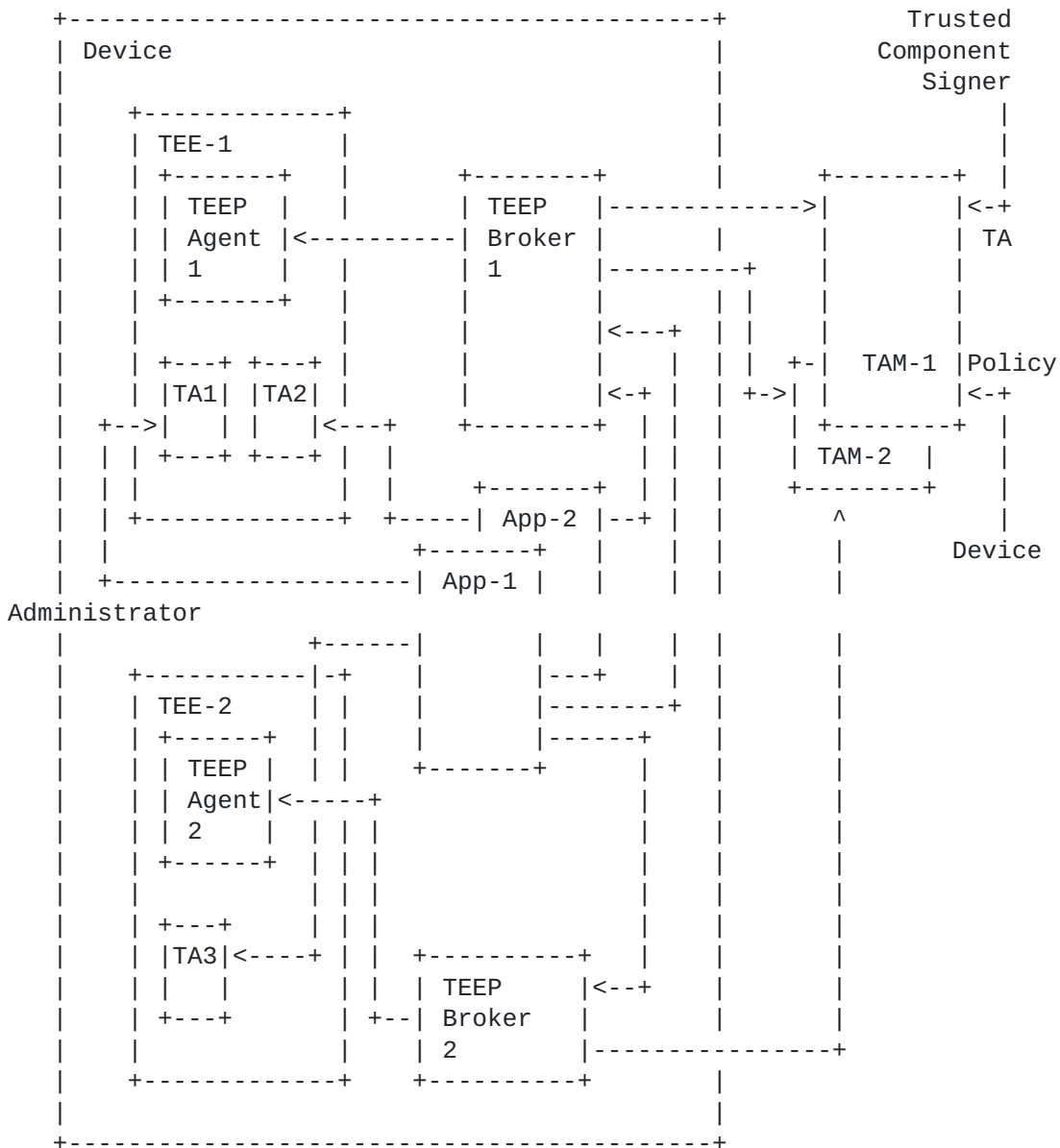
Figure 2: Notional Architecture of TEEP with multiple TEEs
