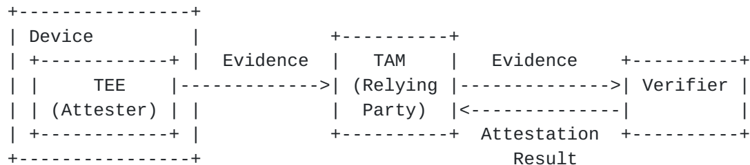
Figure 6: TEEP Attestation Roles
