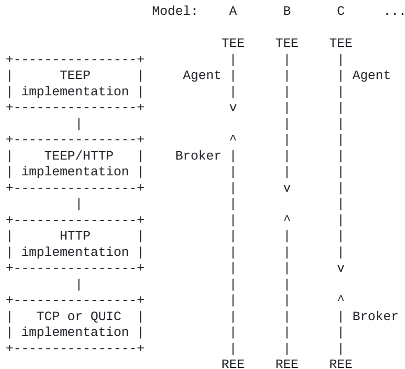
Figure 5: TEEP Broker Models
