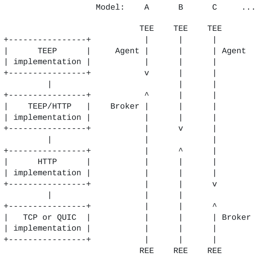
Figure 5: TEEP Broker Models
