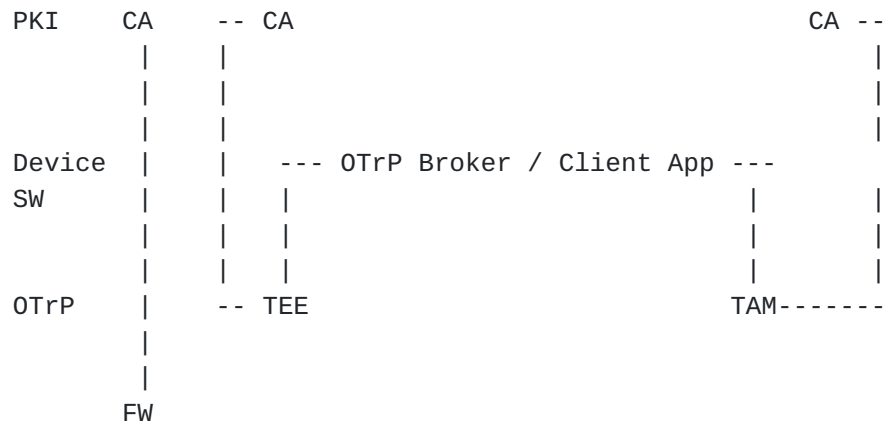
Figure 2: OTrP System Diagram
