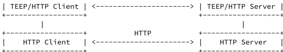
Figure 1: Agent-to-TAM Communication
