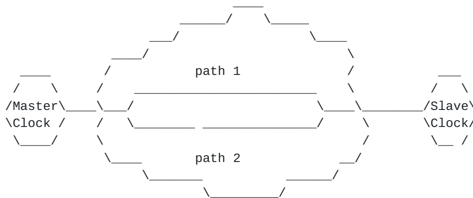
Figure 1 Multi-Path Connection
