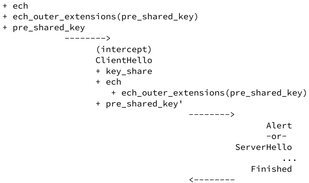
Figure 5: Message flow for malleable ClientHello
