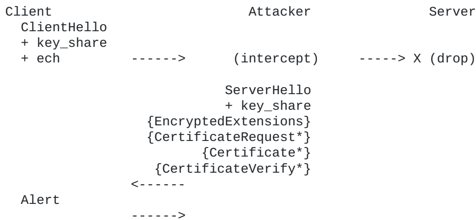
Figure 3: Client reaction attack
