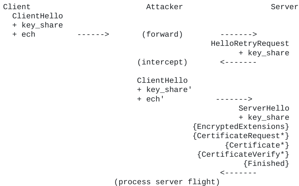
Figure 4: HelloRetryRequest hijack attack
