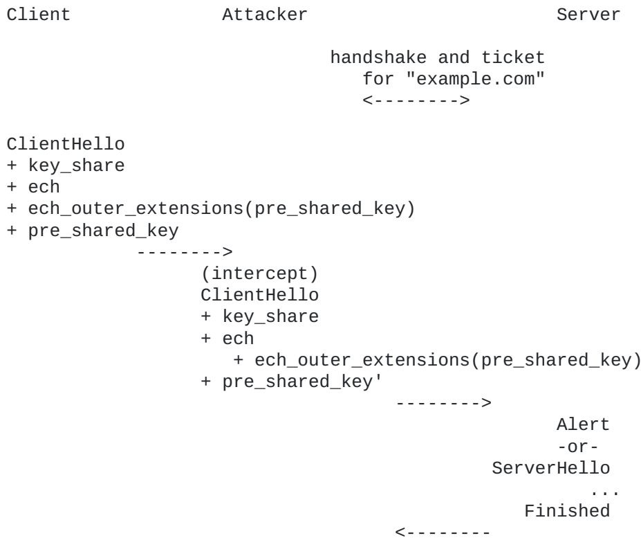
Figure 5: Message flow for malleable ClientHello
