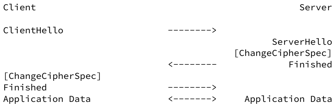
Figure 2 [ RFC5246 ]. Message flow for an abbreviated handshake
