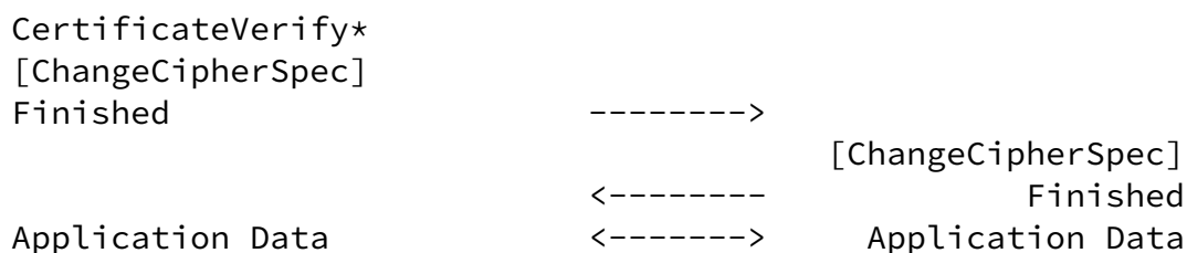
Fig. 1 - Message flow for a full handshake
