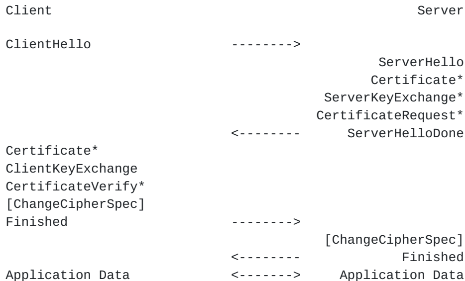
Fig. 1 - Message flow for a full handshake
