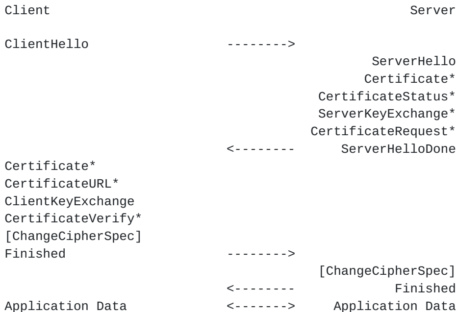
Fig. 1 - Message flow for a full handshake
