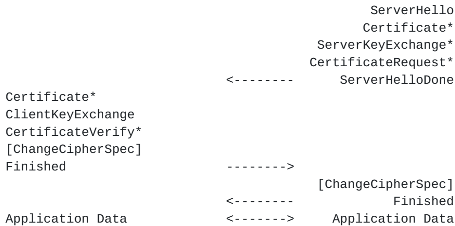
Fig. 1. Message flow for a full handshake
