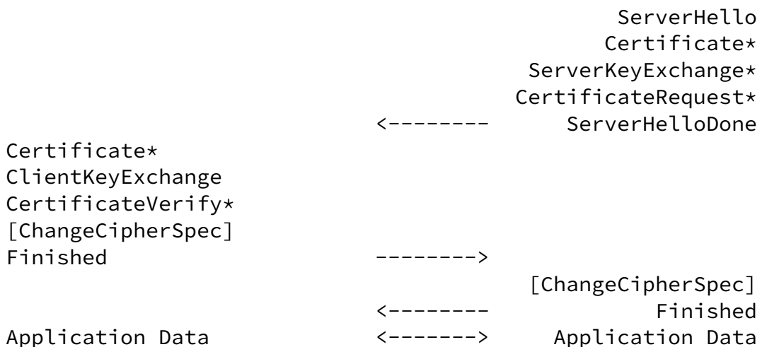
Fig. 1. Message flow for a full handshake
