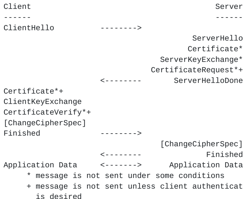
Figure 1: Message flow in a full TLS 1.2 handshake
