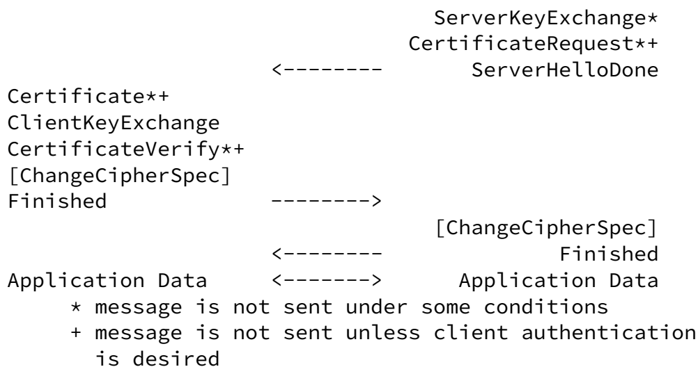
Figure 1: Message flow in a full TLS 1.2 handshake
