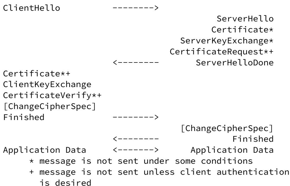
Figure 1: Message flow in a full TLS 1.2 handshake
