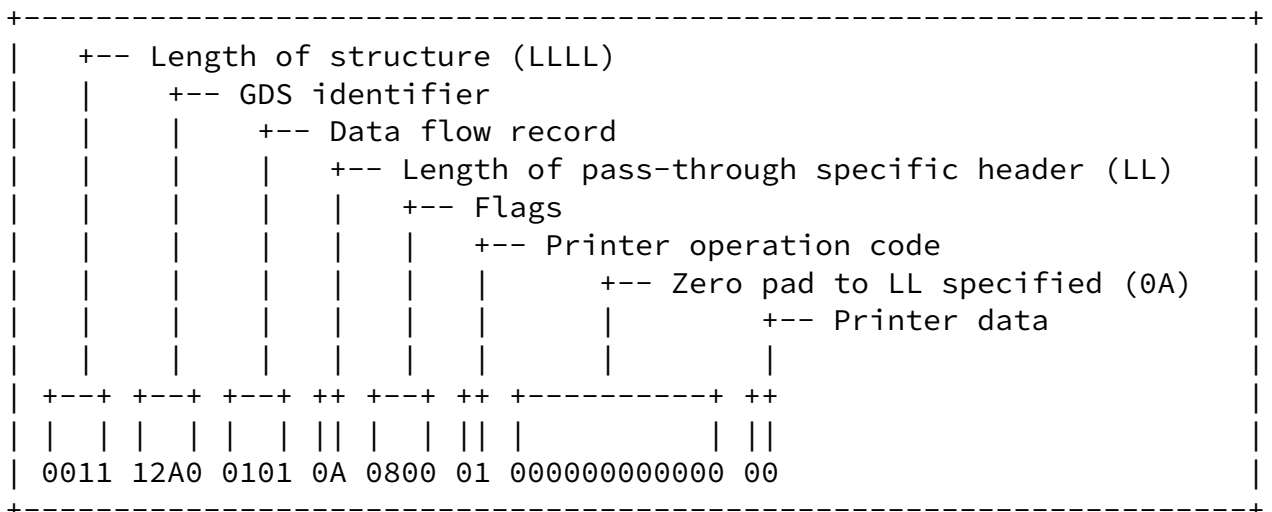
Figure 6. Server sending client a null print record
