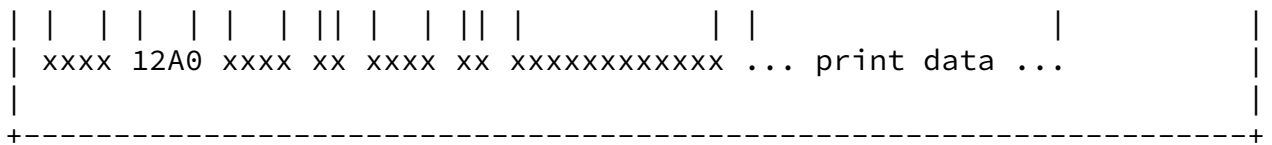
Figure 3. Layout of the printer pass-through header
