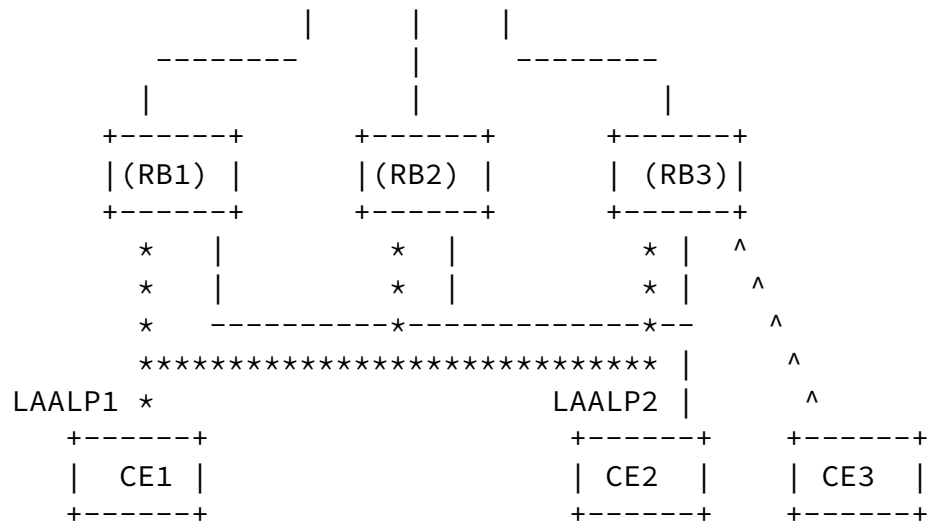
Figure 1 TRILL Active-active access
