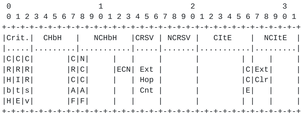
Figure 2. The TRILL-ECN and CCE TRILL Header Extension Flags Word Fields
