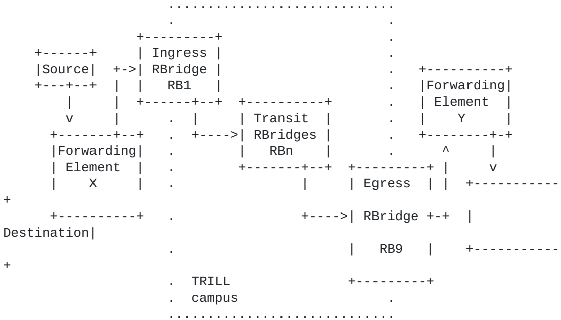
Figure 1. Example Path Forwarding Nodes
