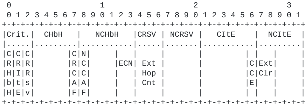
Figure 2. The TRILL-ECN and CCE TRILL Header Extension Flags Word Fields
