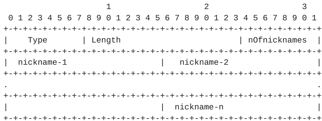
Figure 17 Next Hop RBridge List TLV
