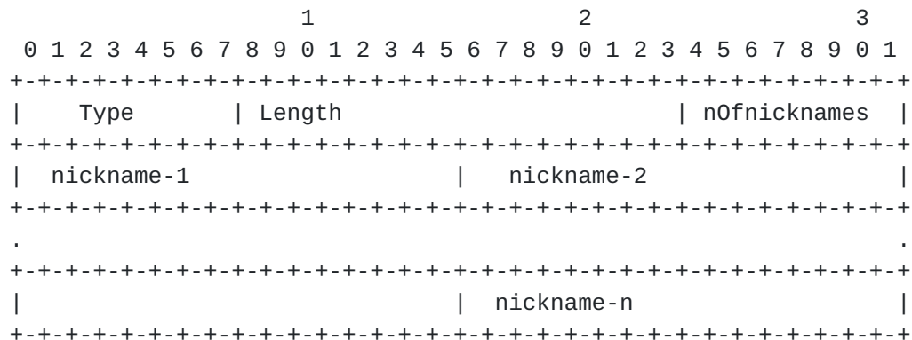
Figure 15 RBridge Scope TLV
