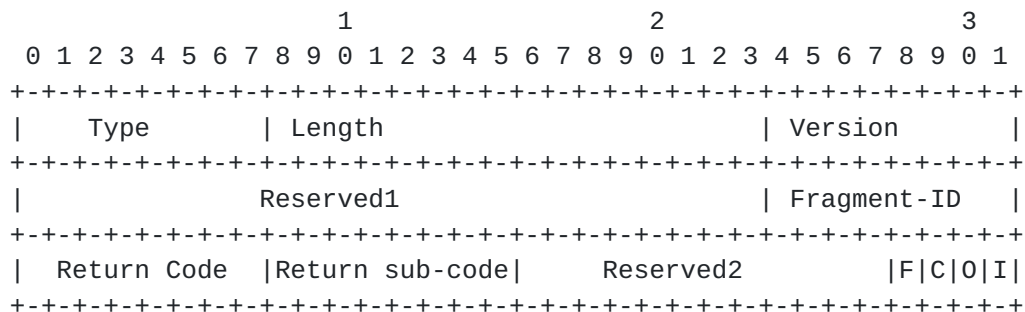
Figure 11 TRILL OAM Application Identifier TLV
