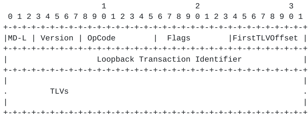
Figure 21 Loopback OAM Message Format
