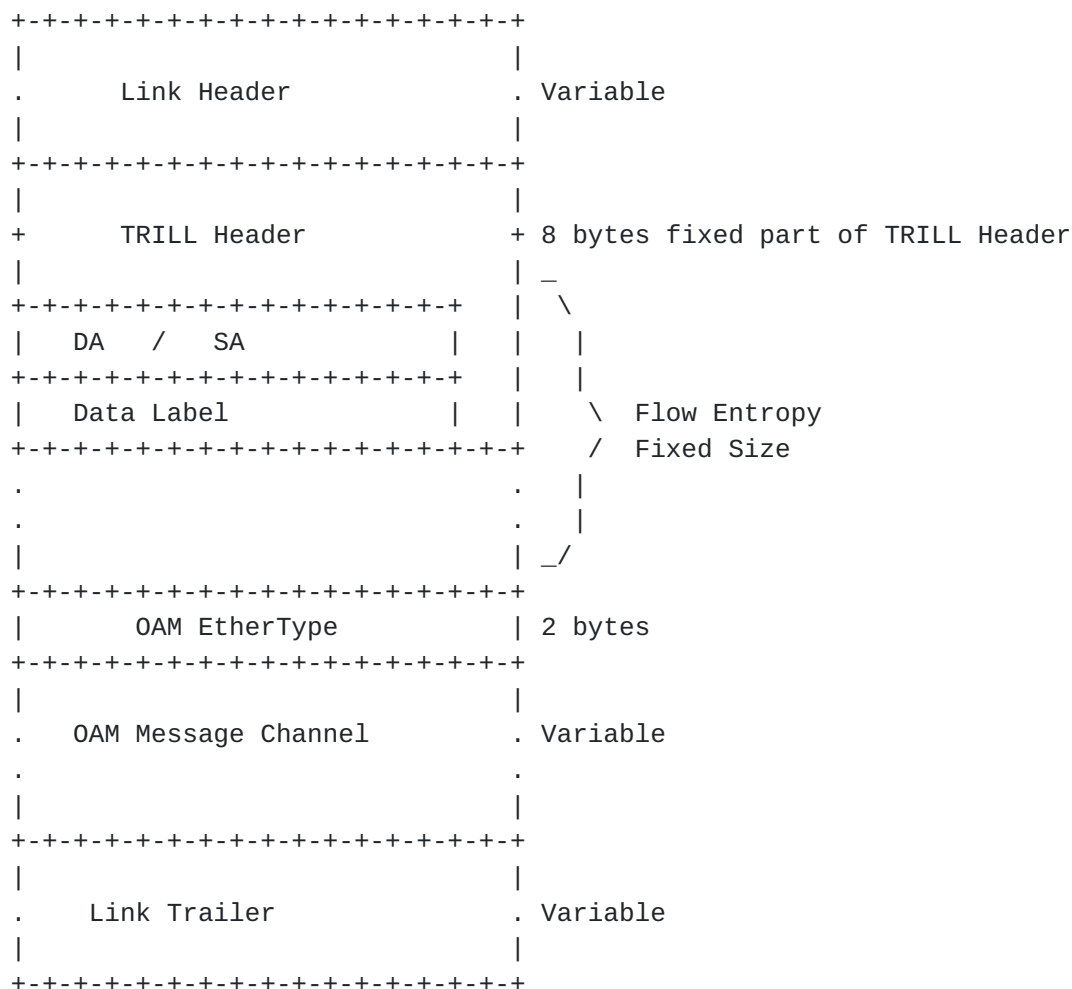
Figure 5: OAM Frame Format
