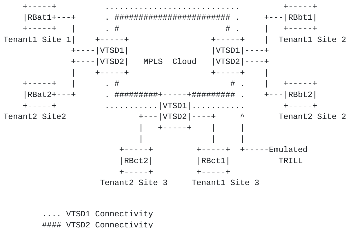
Figure 4: Topological Model of VPTS/TIR connecting 2 tenants with three TRILL Sites
