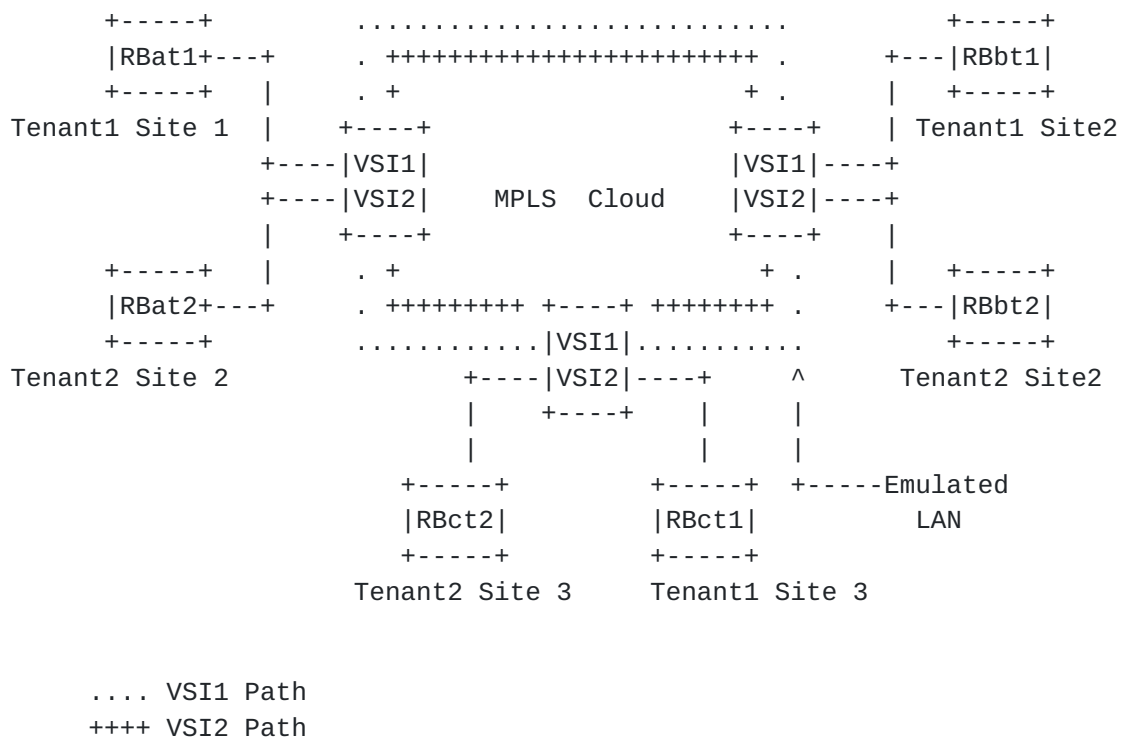
Figure 2: Topological Model for VPLS Model connecting 2 Tenants with 3 sites each
