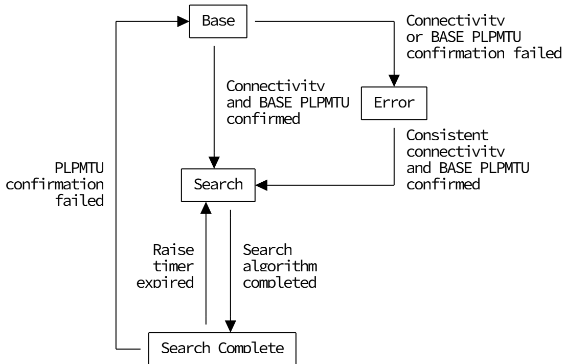
Figure 4: DPLPMTUD Phases
