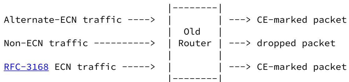
Figure 1: Alternating-ECN traffic, an old router using RFC-3168 ECN.
