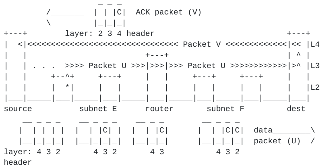
Figure 2: Feed-Up-and-Forward Mode
