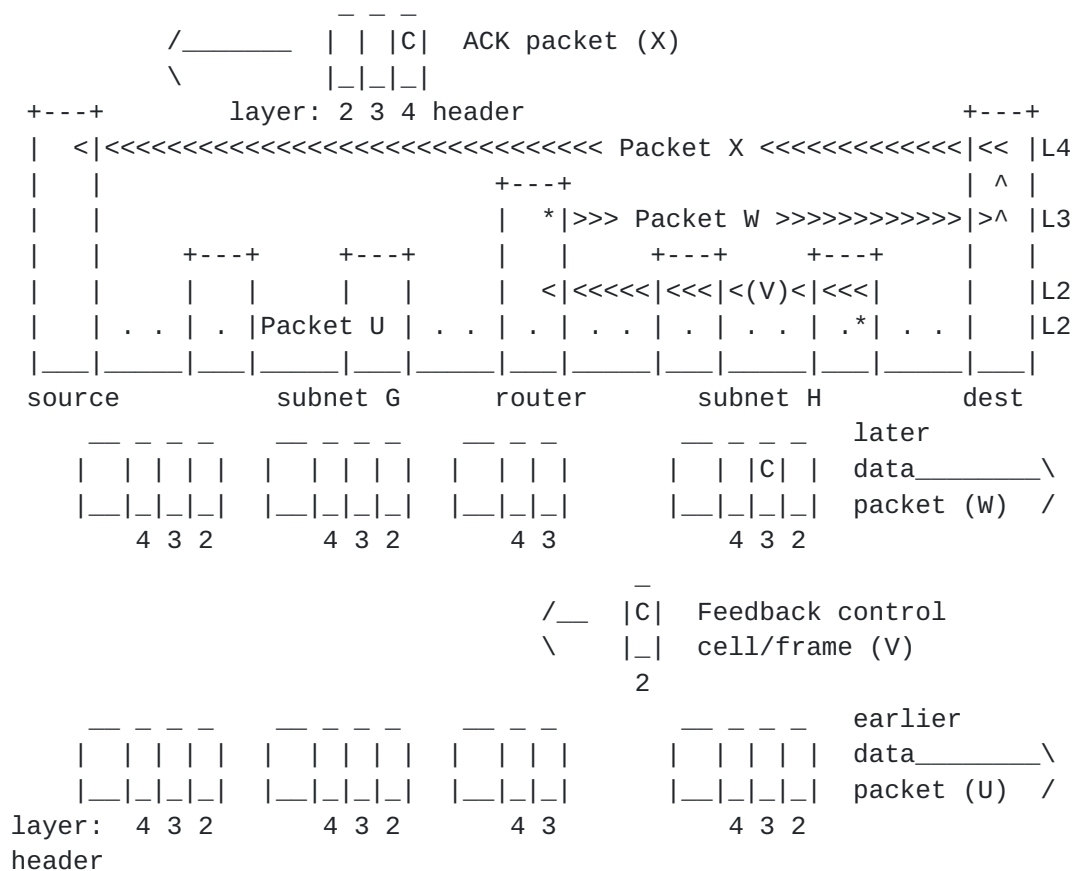
Figure 3: Feed-Backward Mode
